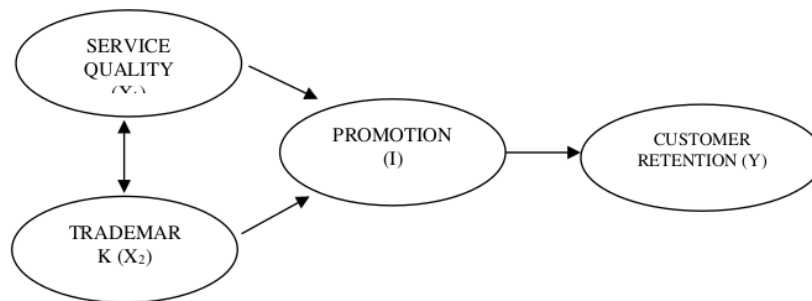
Figure 2.1. Conceptual Framework
